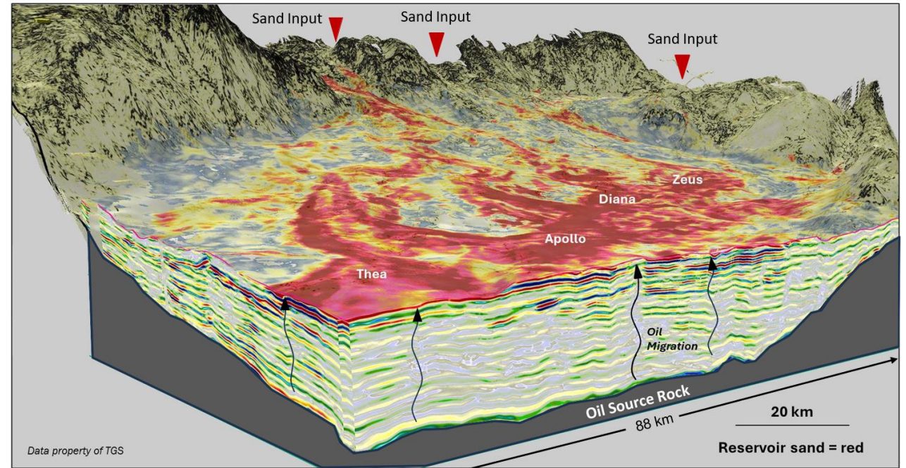
Relative acoustic impedance: Cenomanian top 100 m
