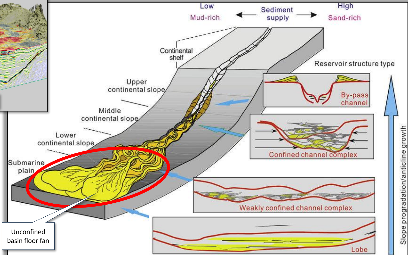
Cenomanian fans in the Harper Basin
